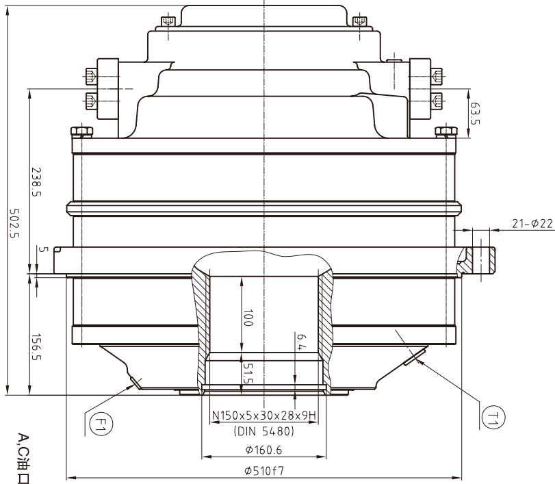
CRM-CA210 外形及安装尺寸/ CRM-CA210 Installation Dimensions
